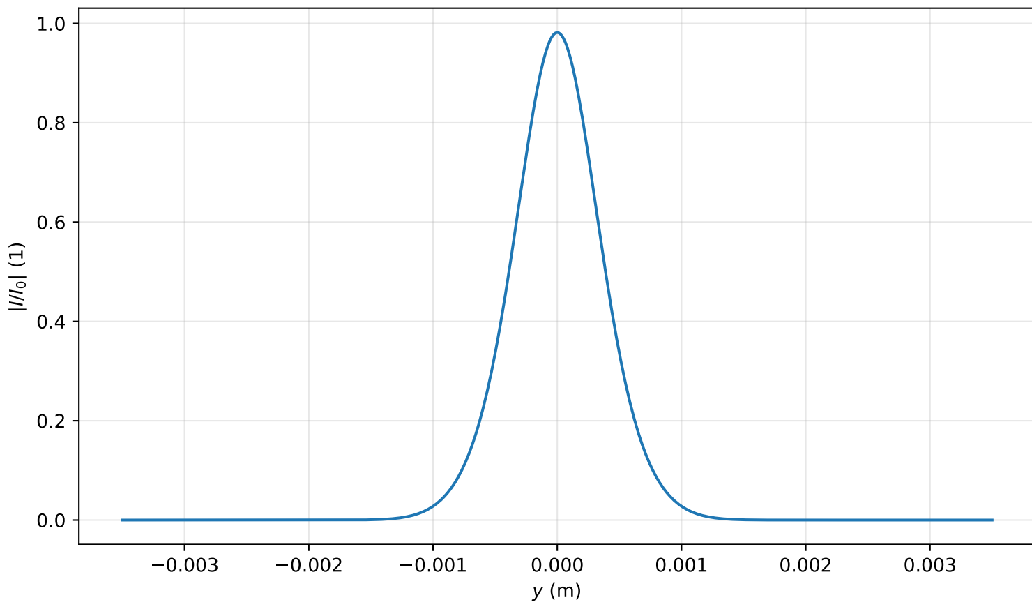
Intensity profile I(x=0, y, z=1.035)/I_0 , \text{Pin}=0.4\text{Pcr} , artificial time
